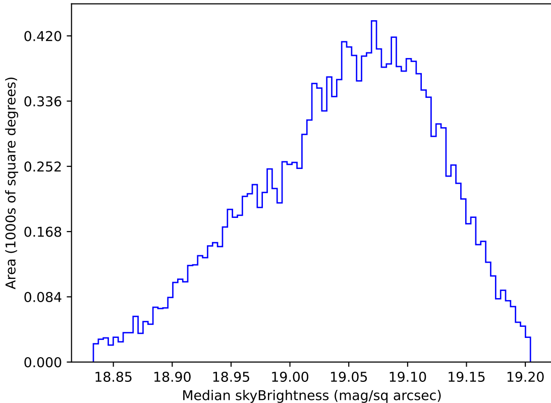
ddf_acor_sf25_lsf30_lsr10_v3.4_10yrs WFD z band: Median skyBrightness
