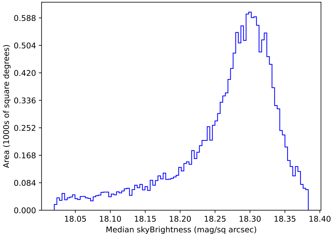
ddf_acor_sf25_lsf30_lsr10_v3.4_10yrs WFD y band: Median skyBrightness
