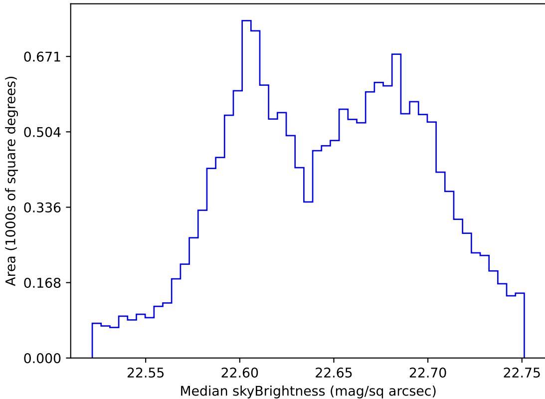
ddf_acor_sf25_lsf30_lsr10_v3.4_10yrs WFD u band: Median skyBrightness
