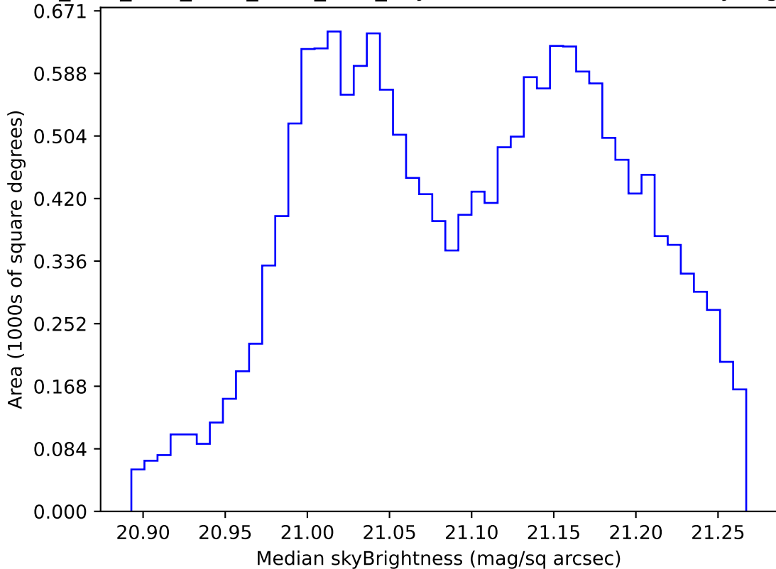
ddf_acor_sf25_lsf30_lsr10_v3.4_10yrs WFD r band: Median skyBrightness
