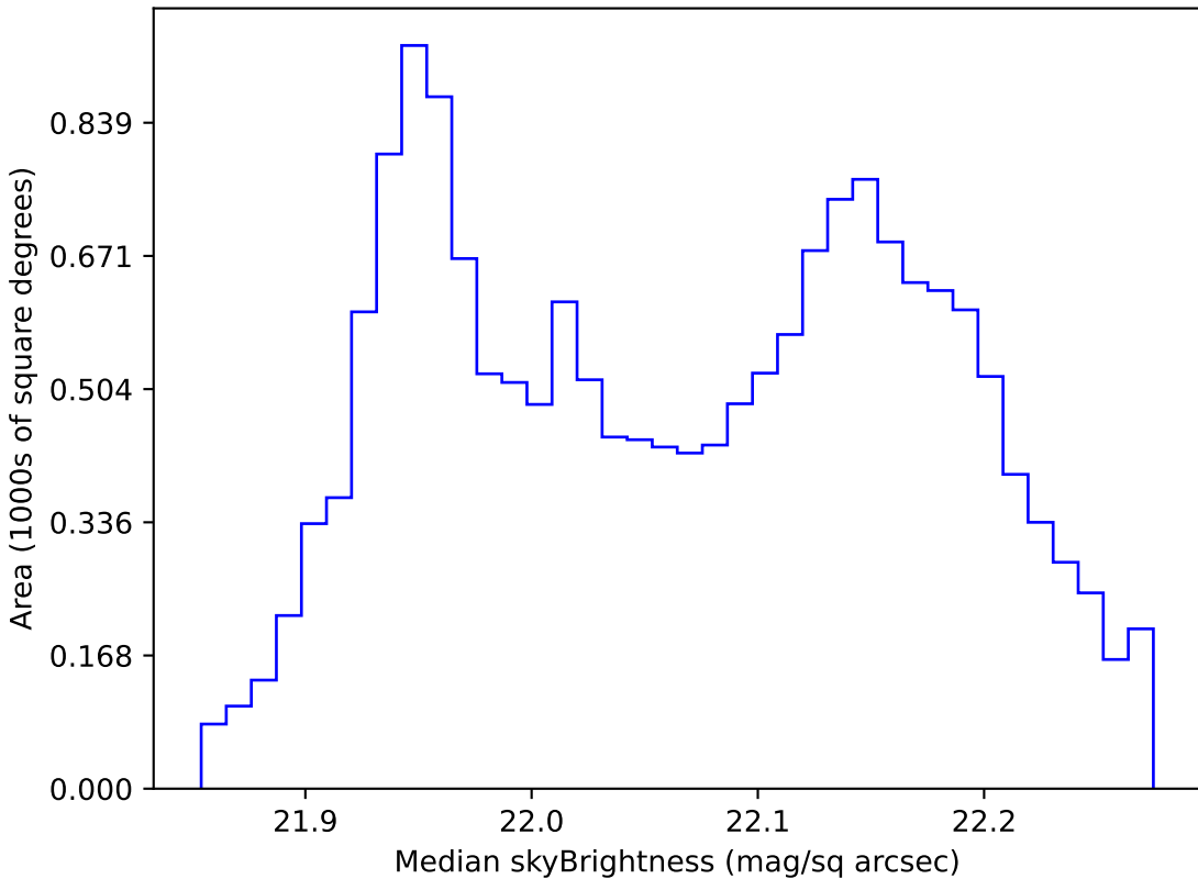
ddf_acor_sf25_lsf30_lsr10_v3.4_10yrs WFD g band: Median skyBrightness
