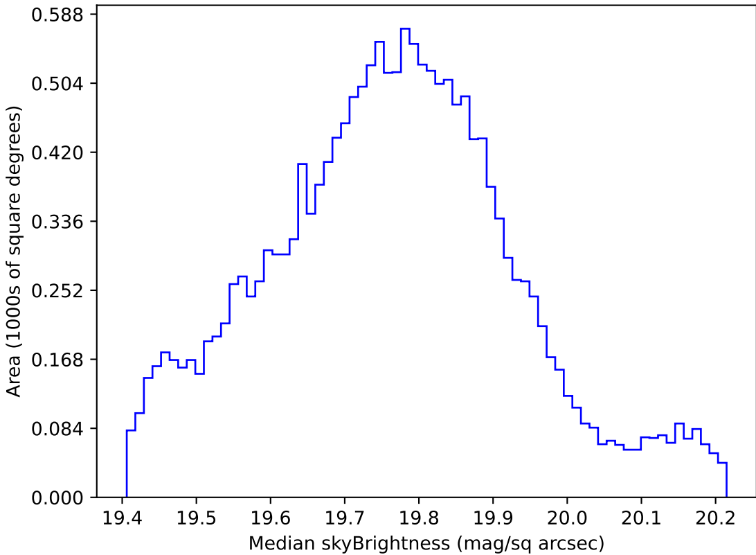
ddf_acor_sf25_lsf30_lsr10_v3.4_10yrs WFD all bands: Median skyBrightness
