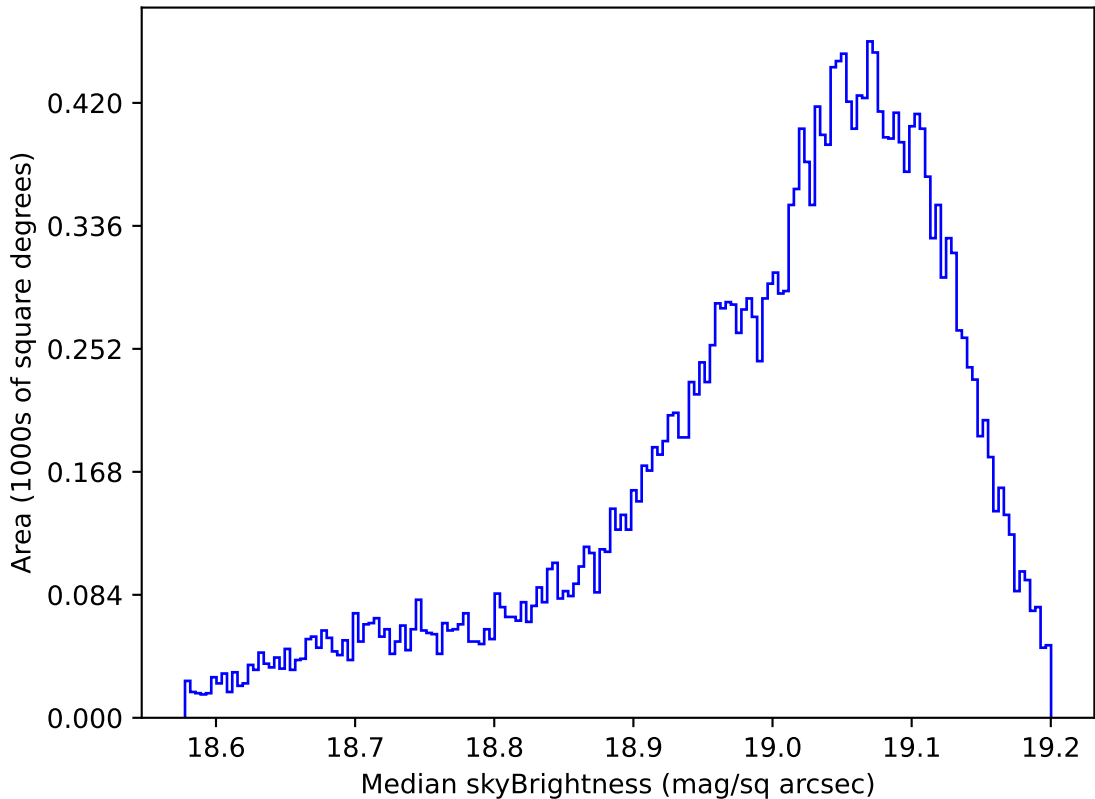
ddf_acor_sf25_lsf30_lsr10_v3.4_10yrs All sky z band: Median skyBrightness
