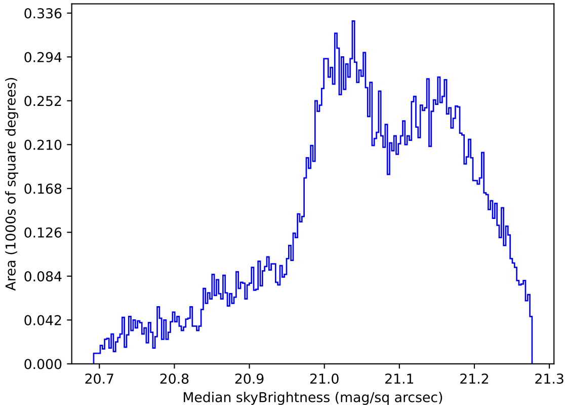
ddf_acor_sf25_lsf30_lsr10_v3.4_10yrs All sky r band: Median skyBrightness
