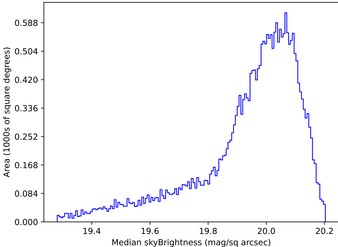
ddf_acor_sf25_lsf30_lsr10_v3.4_10yrs All sky i band: Median skyBrightness
