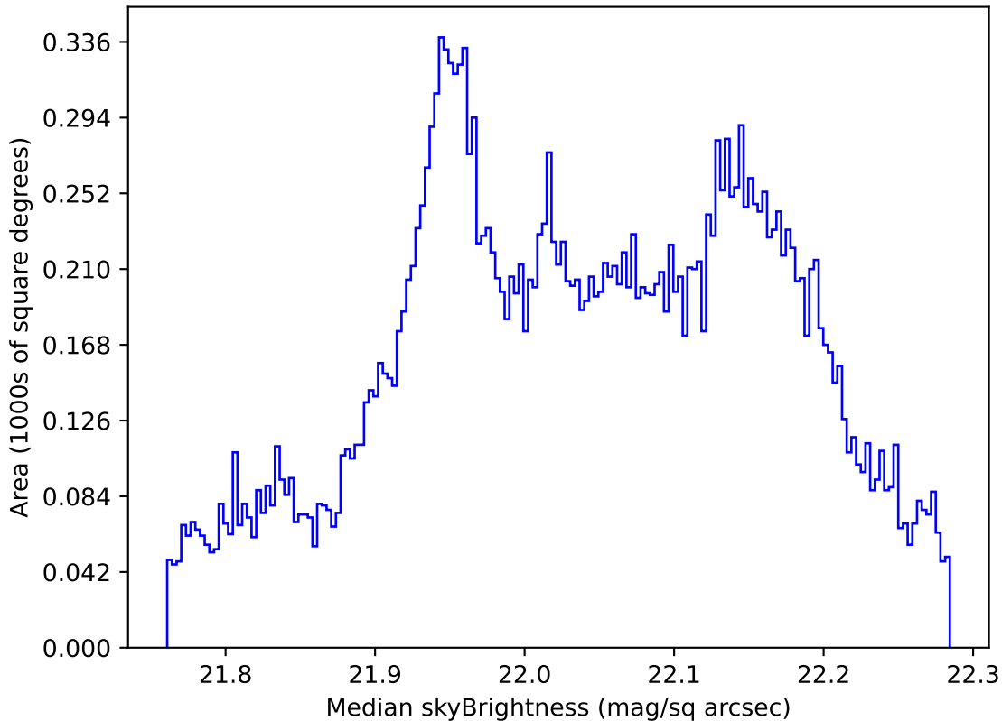
ddf_acor_sf25_lsf30_lsr10_v3.4_10yrs All sky g band: Median skyBrightness
