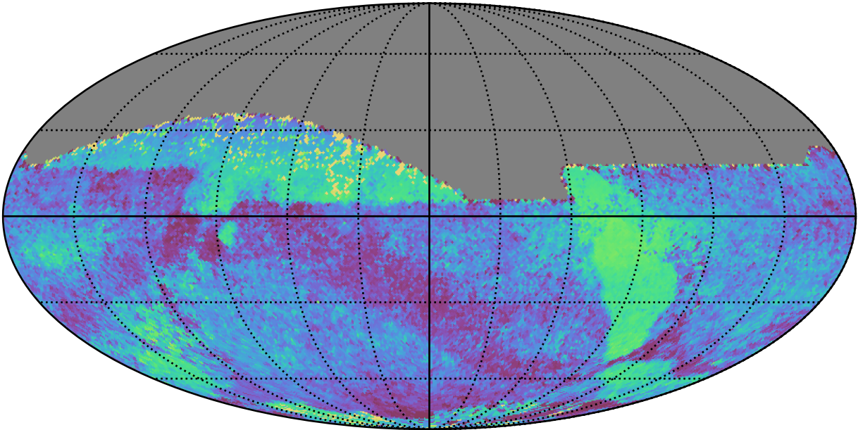
ddf_acor_sf25_lsf30_lsr10_v3.4_10yrs All sky all bands: Median skyBrightness
