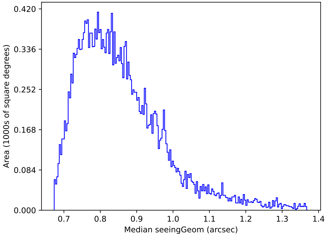
ddf_acor_sf25_lsf30_lsr10_v3.4_10yrs Yr 1 z band: Median seeingGeom
