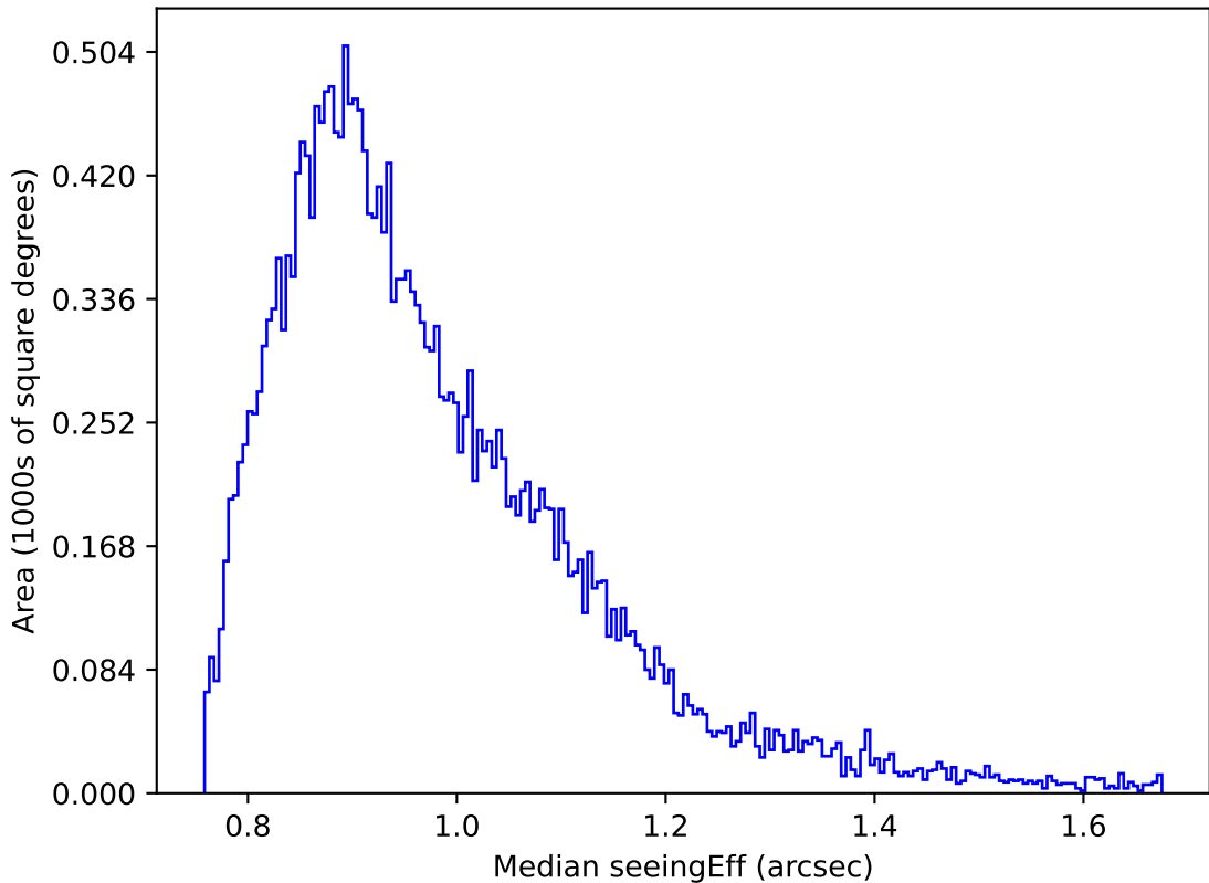
ddf_acor_sf25_lsf30_lsr10_v3.4_10yrs Yr 1 r band: Median seeingEff
