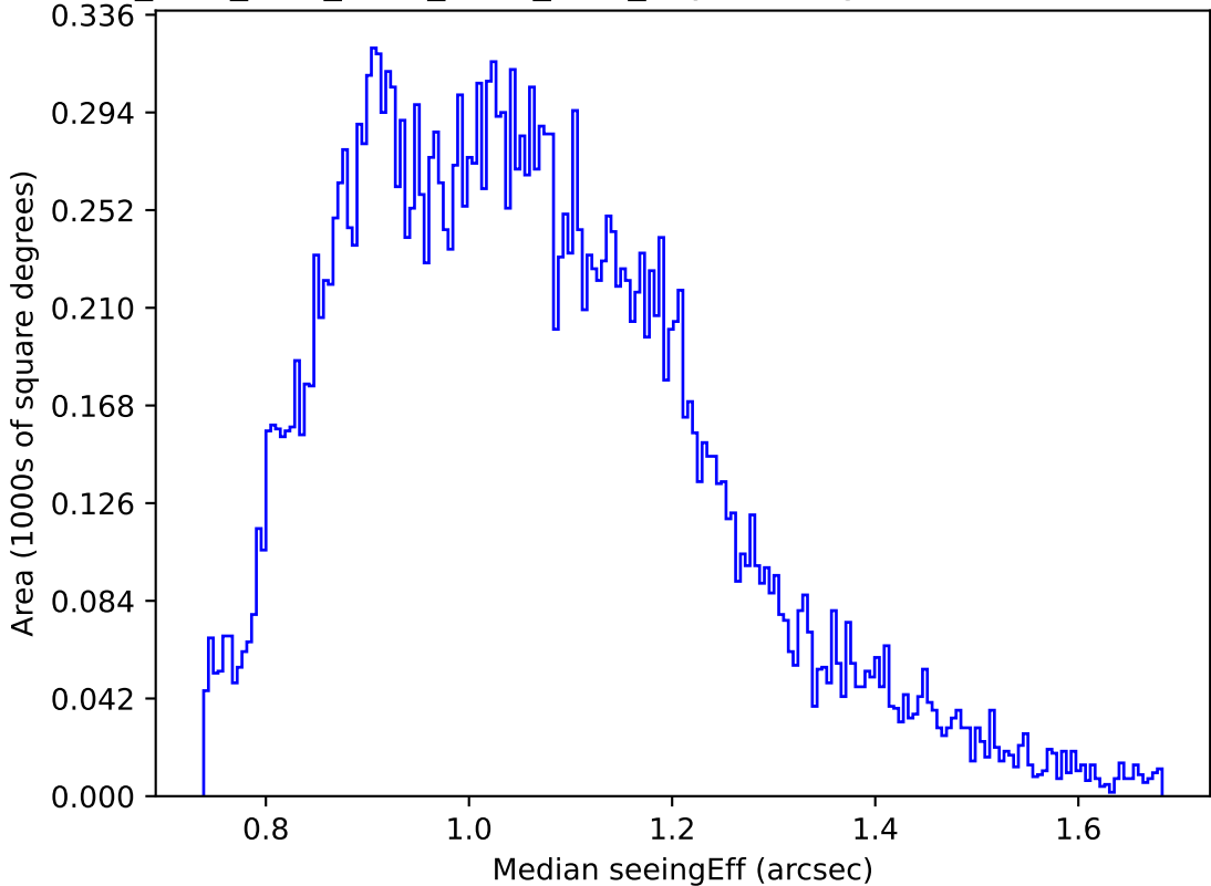
ddf_acor_sf25_lsf30_lsr10_v3.4_10yrs Yr 1 g band: Median seeingEff
