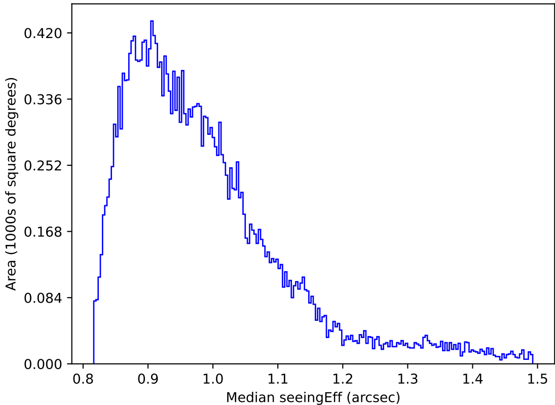
ddf_acor_sf25_lsf30_lsr10_v3.4_10yrs Yr 1 all bands: Median seeingEff
