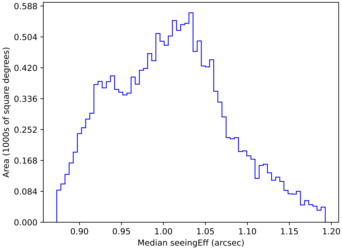
ddf_acor_sf25_lsf30_lsr10_v3.4_10yrs WFD z band: Median seeingEff
