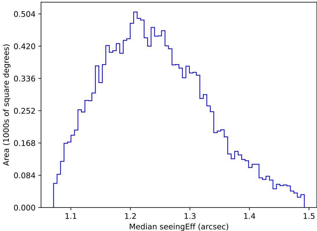
ddf_acor_sf25_lsf30_lsr10_v3.4_10yrs WFD u band: Median seeingEff
