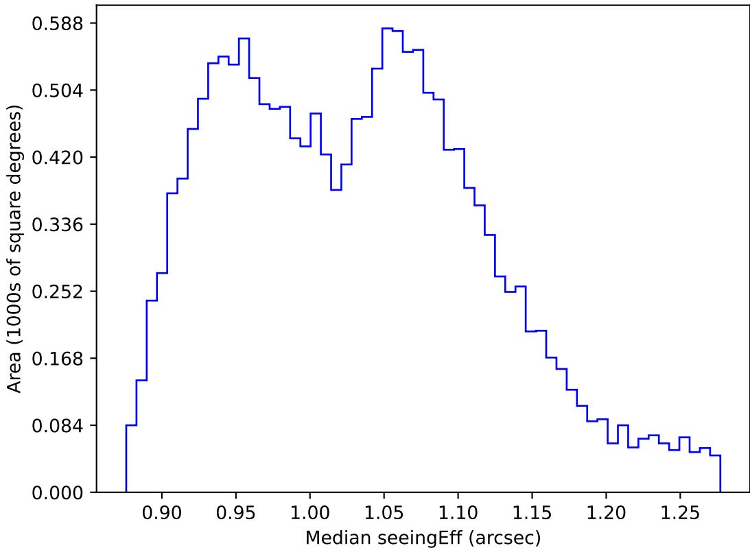
ddf_acor_sf25_lsf30_lsr10_v3.4_10yrs WFD r band: Median seeingEff
