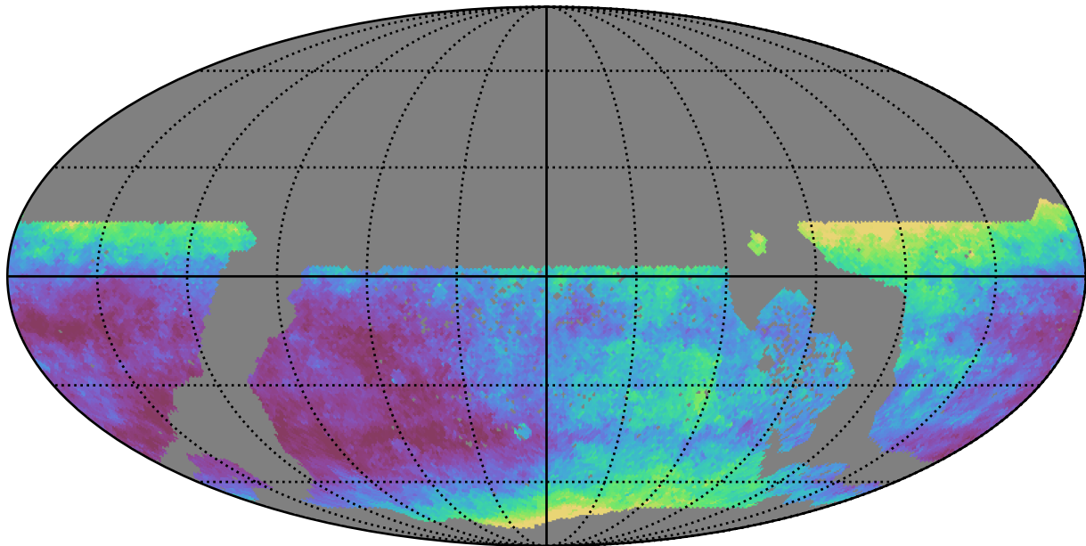
ddf_acor_sf25_lsf30_lsr10_v3.4_10yrs WFD i band: Median seeingEff
