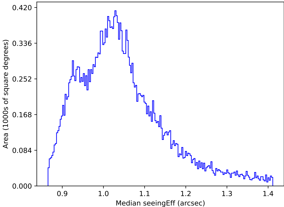
ddf_acor_sf25_lsf30_lsr10_v3.4_10yrs All sky z band: Median seeingEff
