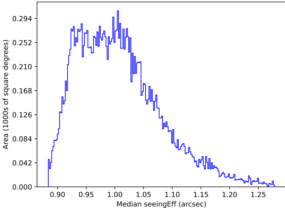
ddf_acor_sf25_ls30_lsr10_v3.4_10yrs All sky y band: Median seeingEff
