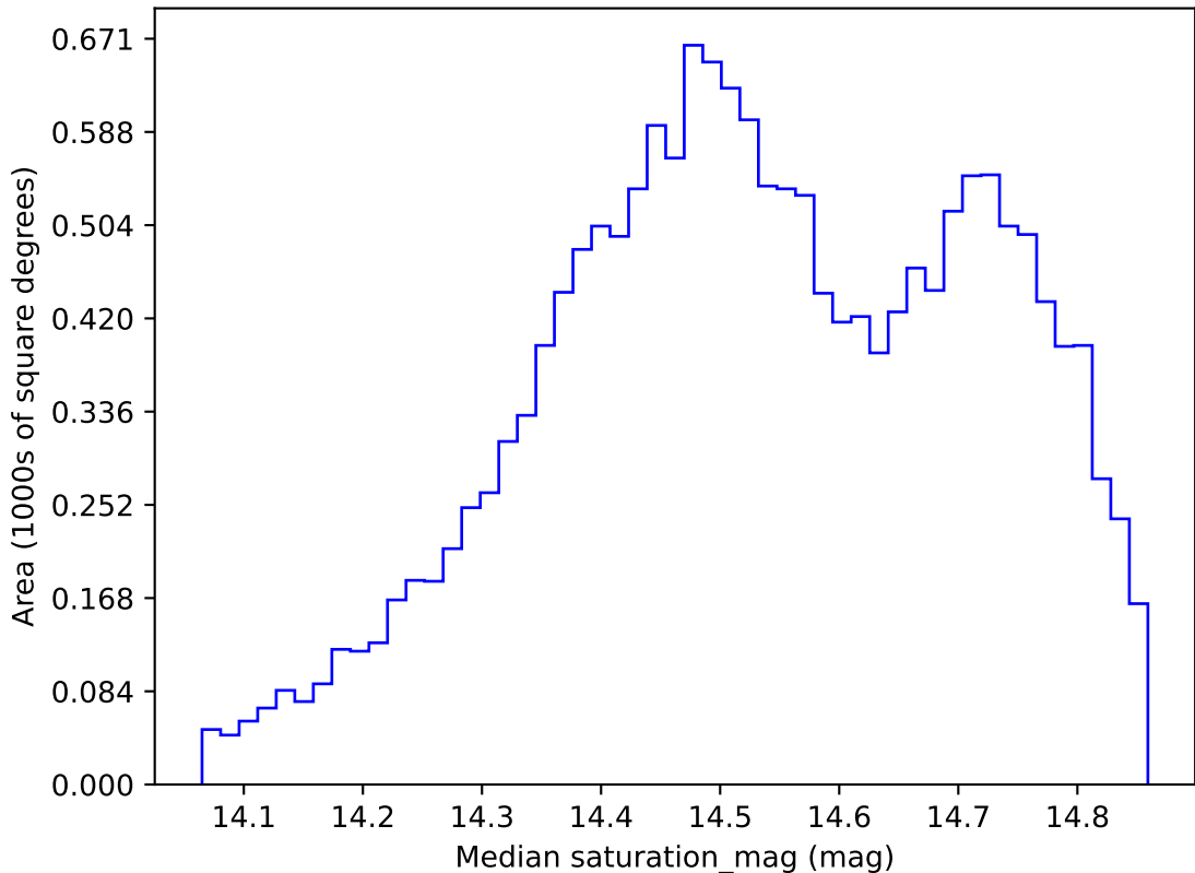
ddf_acor_sf25_lsf30_lsr10_v3.4_10yrs WFD i band: Median saturation_mag
