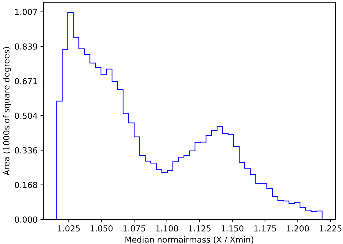
ddf_acor_sf25_lsf30_lsr10_v3.4_10yrs WFD g band: Median normairmass
