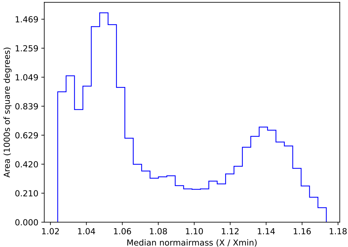
ddf_acor_sf25_lsf30_lsr10_v3.4_10yrs WFD all bands: Median normairmass
