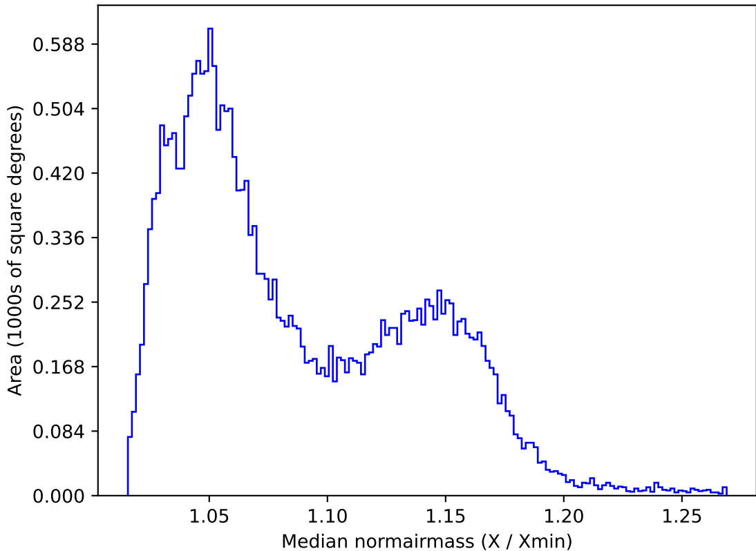
ddf_acor_sf25_lsf30_lsr10_v3.4_10yrs All sky z band: Median normairmass
