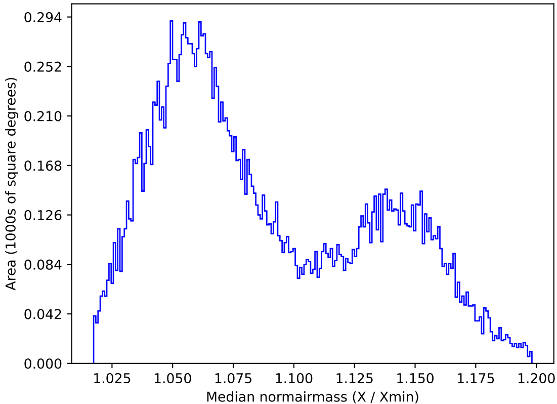
ddf_acor_sf25_lsf30_lsr10_v3.4_10yrs All sky y band: Median normairmass
