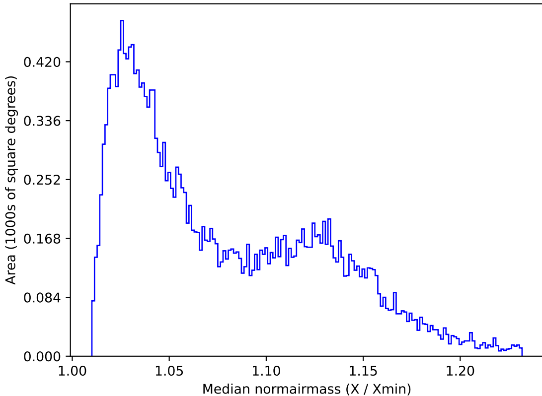
ddf_acor_sf25_lsf30_lsr10_v3.4_10yrs All sky u band: Median normairmass
