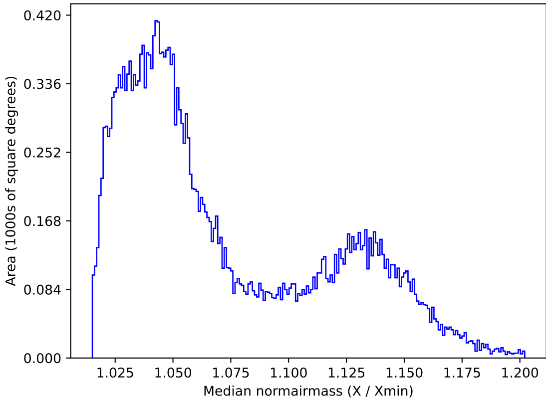
ddf_acor_sf25_lsf30_lsr10_v3.4_10yrs All sky r band: Median normairmass
