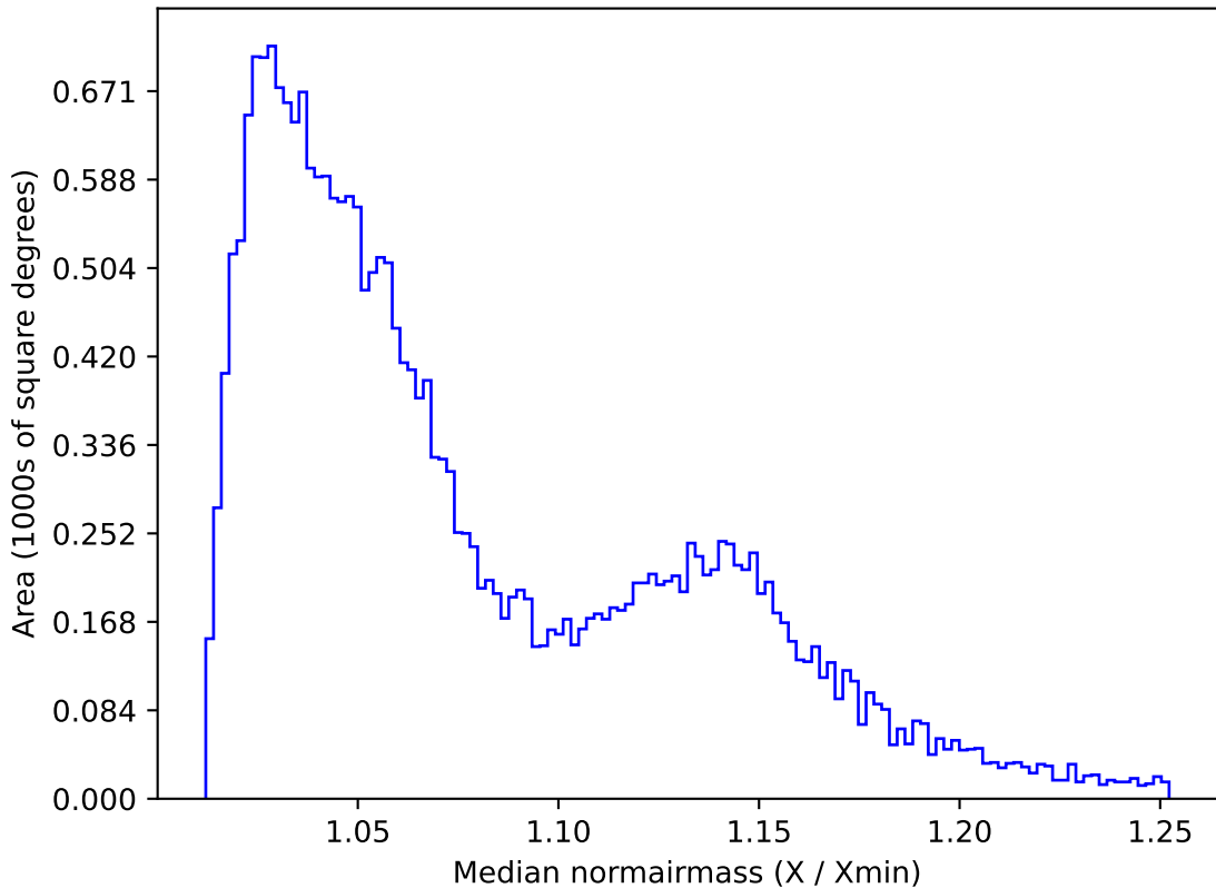
ddf_acor_sf25_lsf30_lsr10_v3.4_10yrs All sky g band: Median normairmass
