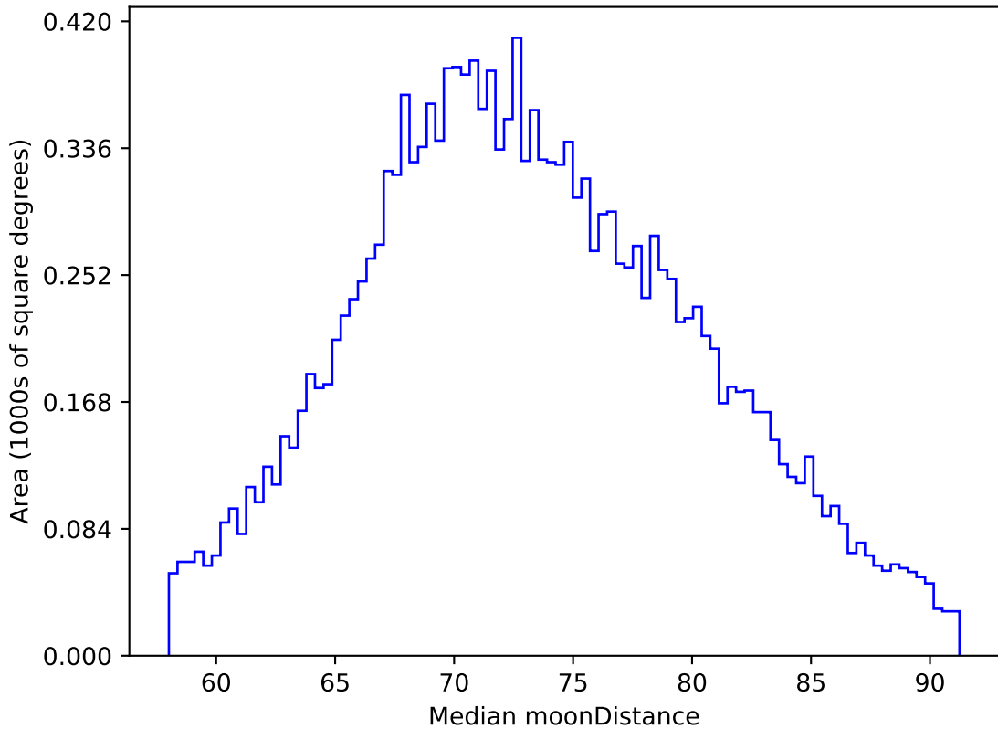
ddf_acor_sf25_lsf30_lsr10_v3.4_10yrs WFD z band: Median moonDistance
