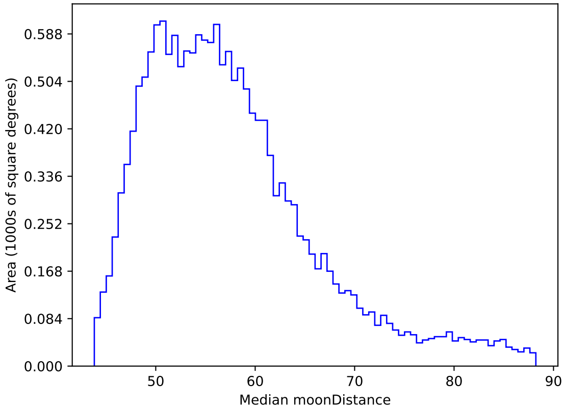
ddf_acor_sf25_lsf30_lsr10_v3.4_10yrs WFD y band: Median moonDistance
