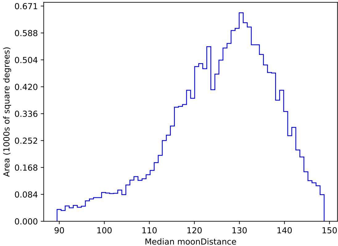
ddf_acor_sf25_lsf30_lsr10_v3.4_10yrs WFD u band: Median moonDistance
