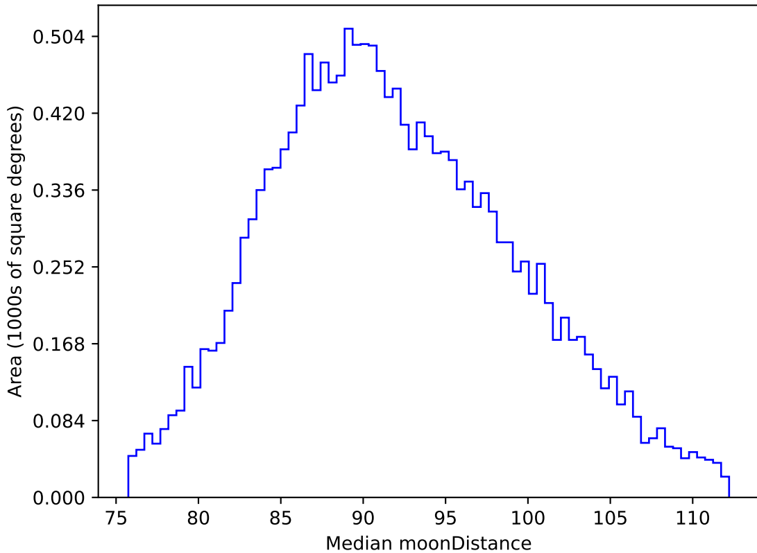
ddf_acor_sf25_lsf30_lsr10_v3.4_10yrs WFD i band: Median moonDistance
