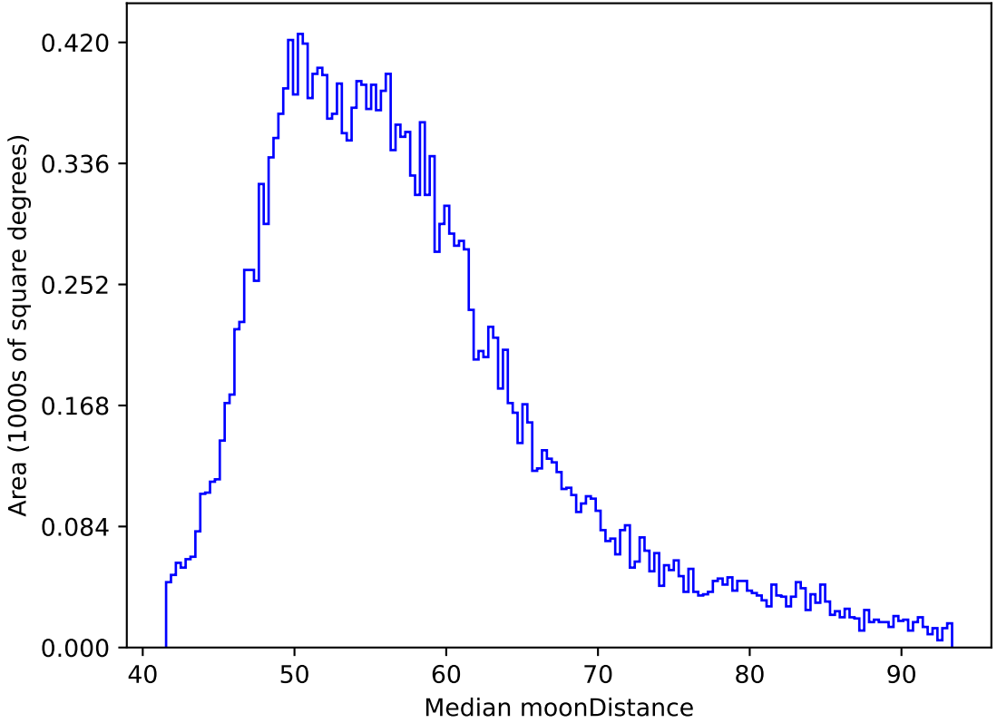
ddf_acor_sf25_lsf30_lsr10_v3.4_10yrs All sky y band: Median moonDistance
