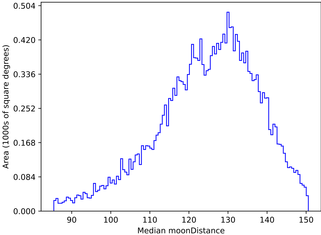
ddf_acor_sf25_lsf30_lsr10_v3.4_10yrs All sky u band: Median moonDistance
