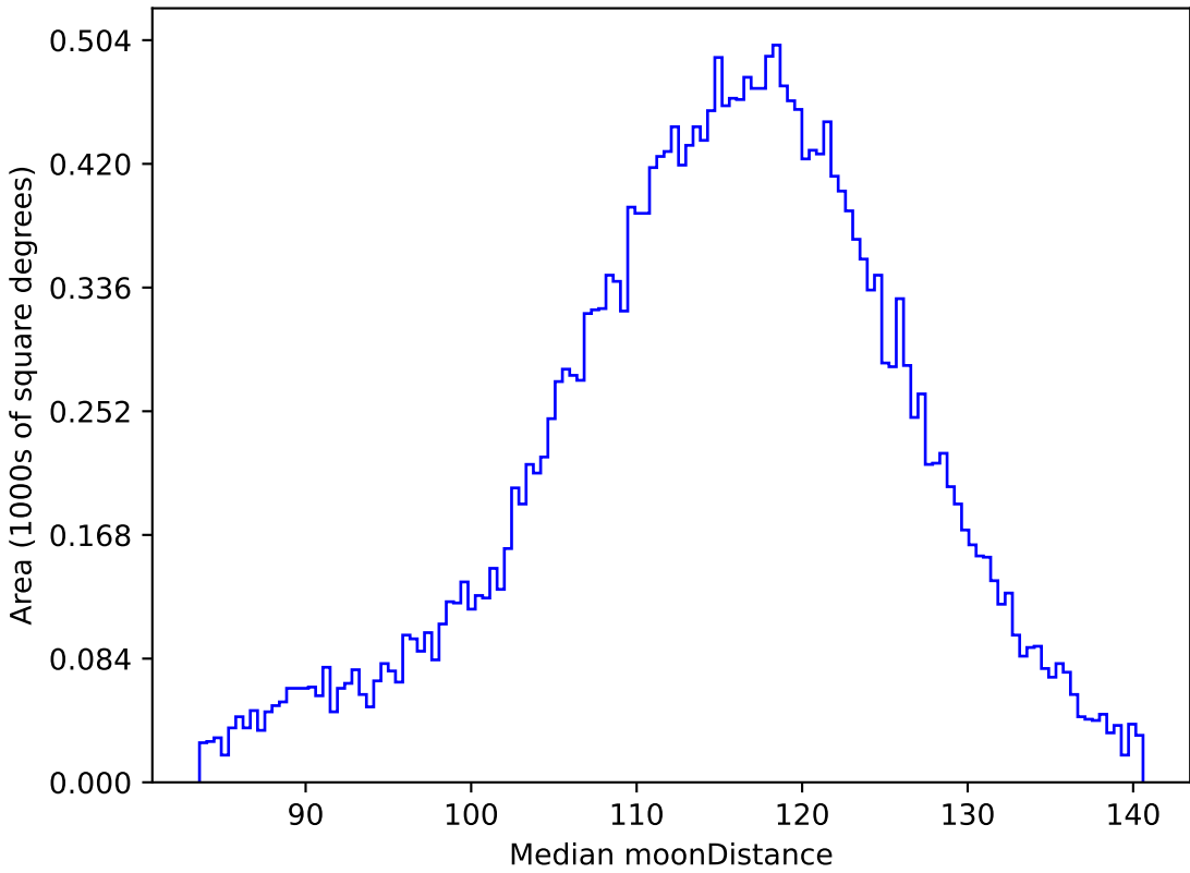
ddf_acor_sf25_lsf30_lsr10_v3.4_10yrs All sky g band: Median moonDistance
