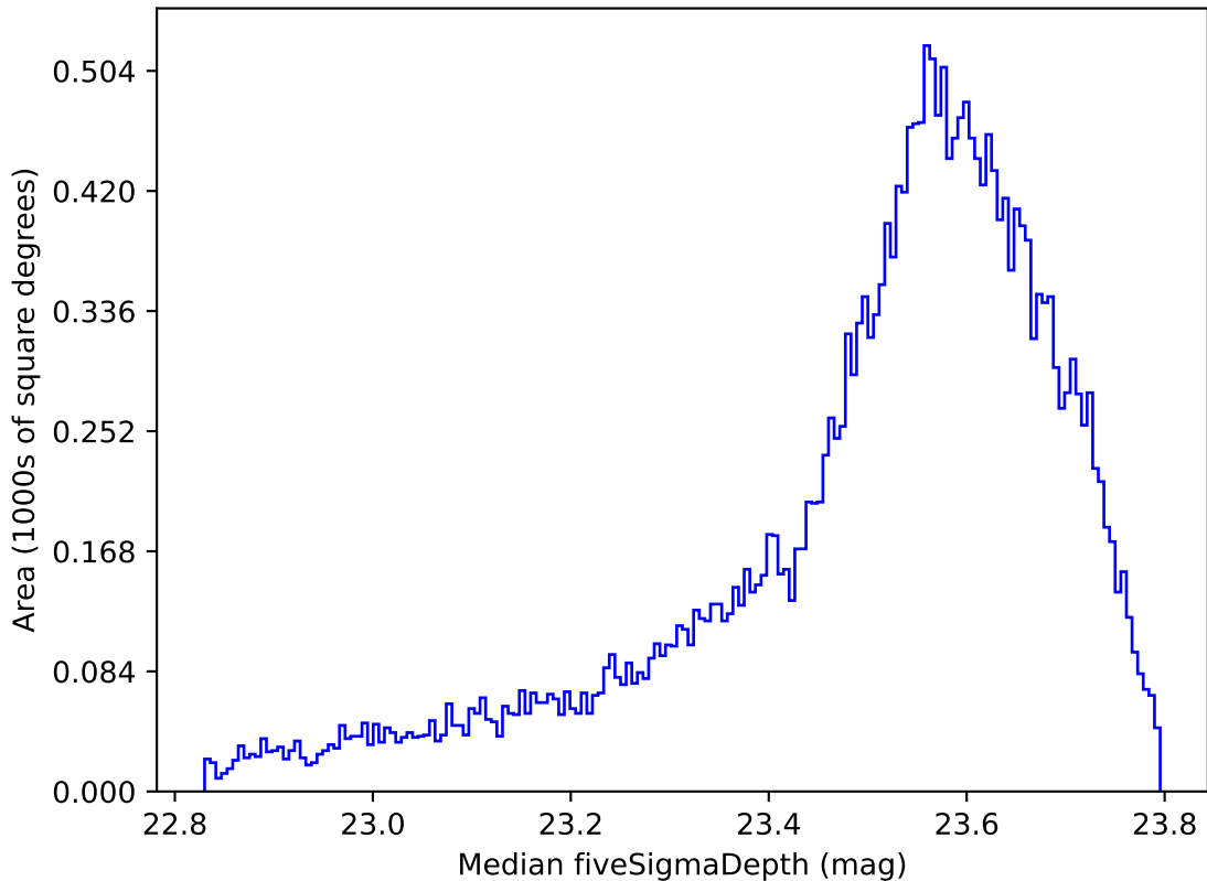
ddf_acor_sf25_lsf30_lsr10_v3.4_10yrs All sky i band: Median fiveSigmaDepth
