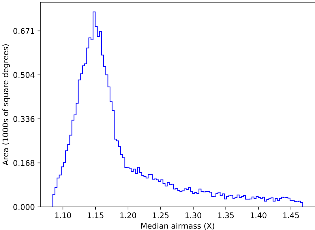
ddf_acor_sf25_lsf30_lsr10_v3.4_10yrs WFD z band: Median airmass
