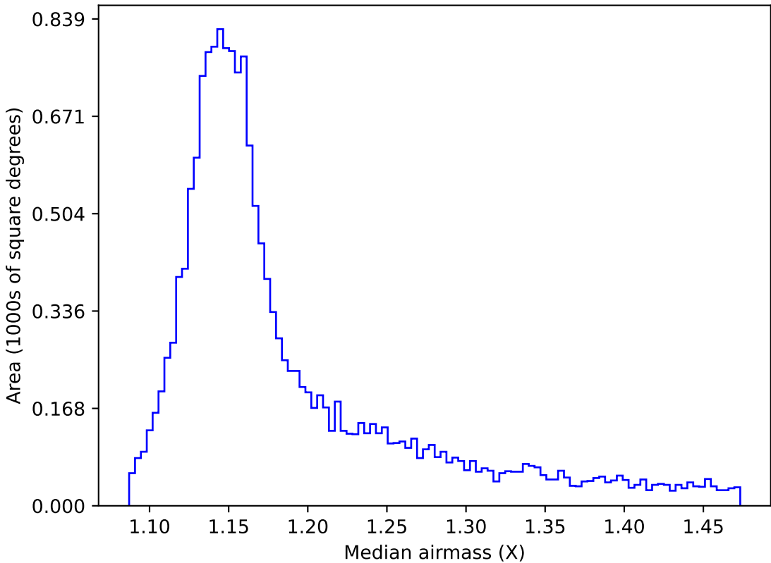
ddf_acor_sf25_lsf30_lsr10_v3.4_10yrs WFD y band: Median airmass
