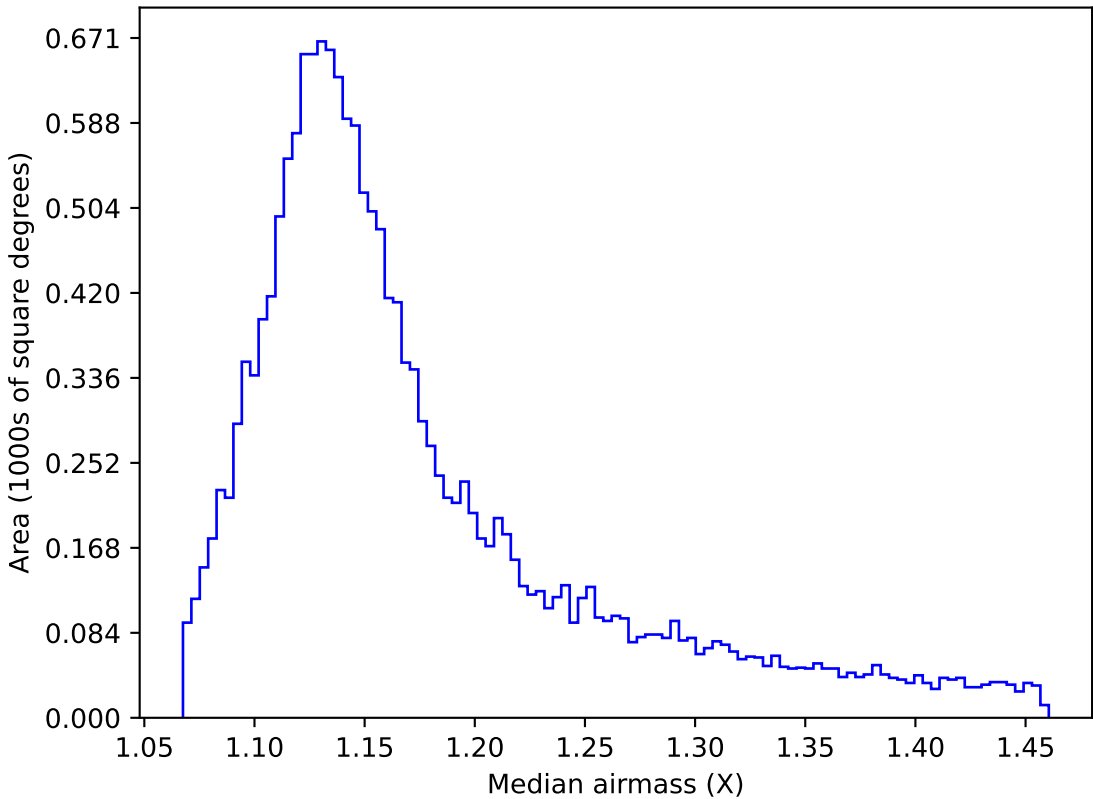
ddf_acor_sf25_lsf30_lsr10_v3.4_10yrs WFD u band: Median airmass
