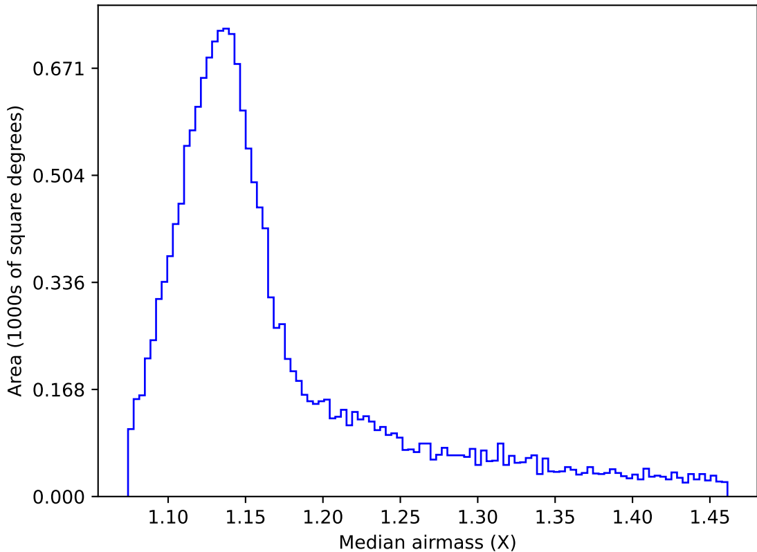
ddf_acor_sf25_lsf30_lsr10_v3.4_10yrs WFD r band: Median airmass
