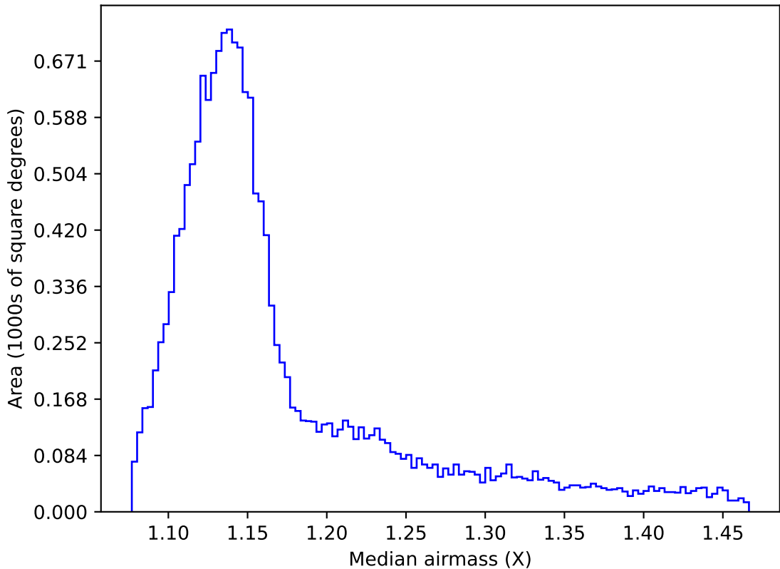
ddf_acor_sf25_lsf30_lsr10_v3.4_10yrs WFD i band: Median airmass
