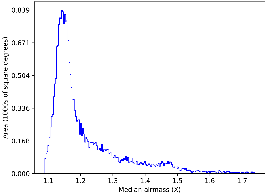
ddf_acor_sf25_lsf30_lsr10_v3.4_10yrs All sky y band: Median airmass
