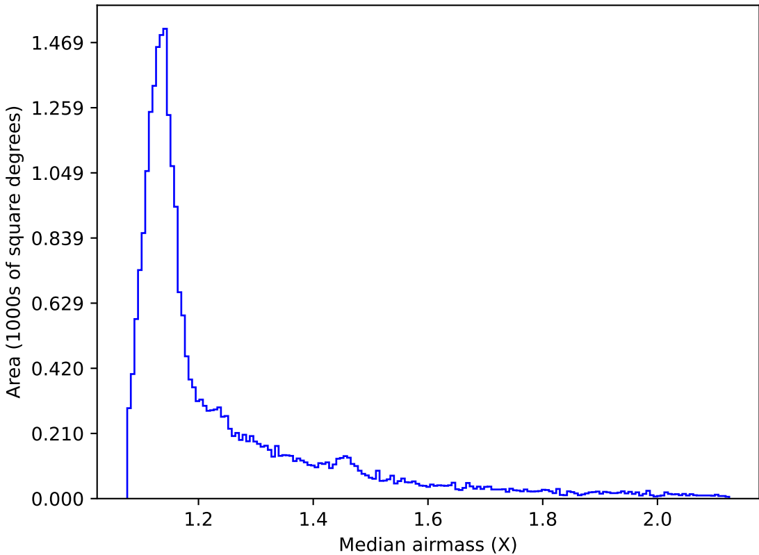
ddf_acor_sf25_lsf30_lsr10_v3.4_10yrs All sky r band: Median airmass
