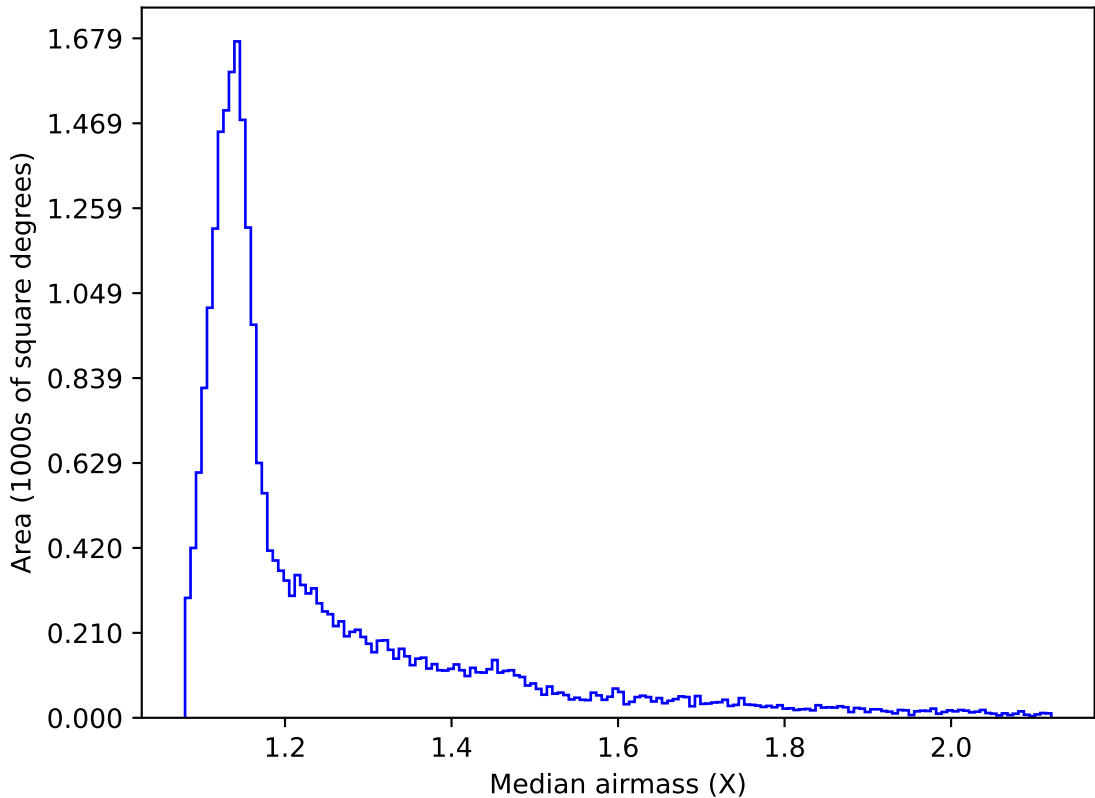
ddf_acor_sf25_lsf30_lsr10_v3.4_10yrs All sky i band: Median airmass
