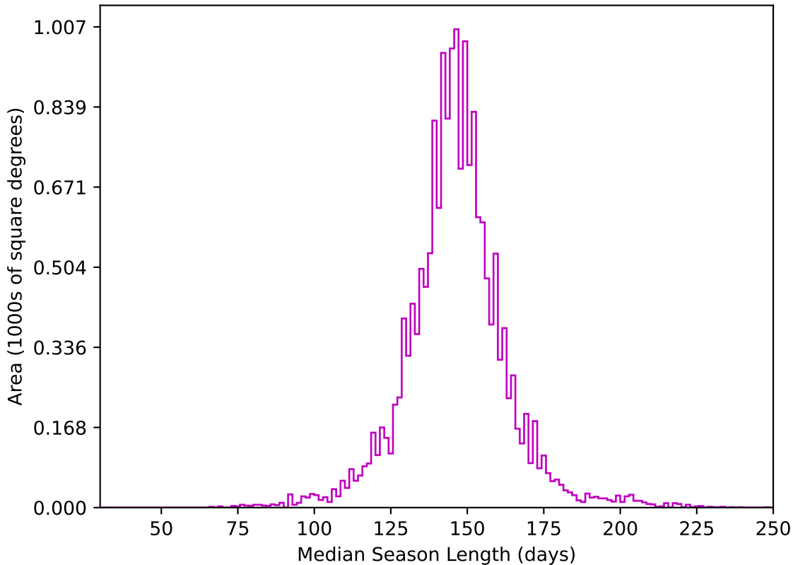
ddf_acor_sf25_lsf30_lsr10_v3.4_10yrs WFD z band: Median Season Length
