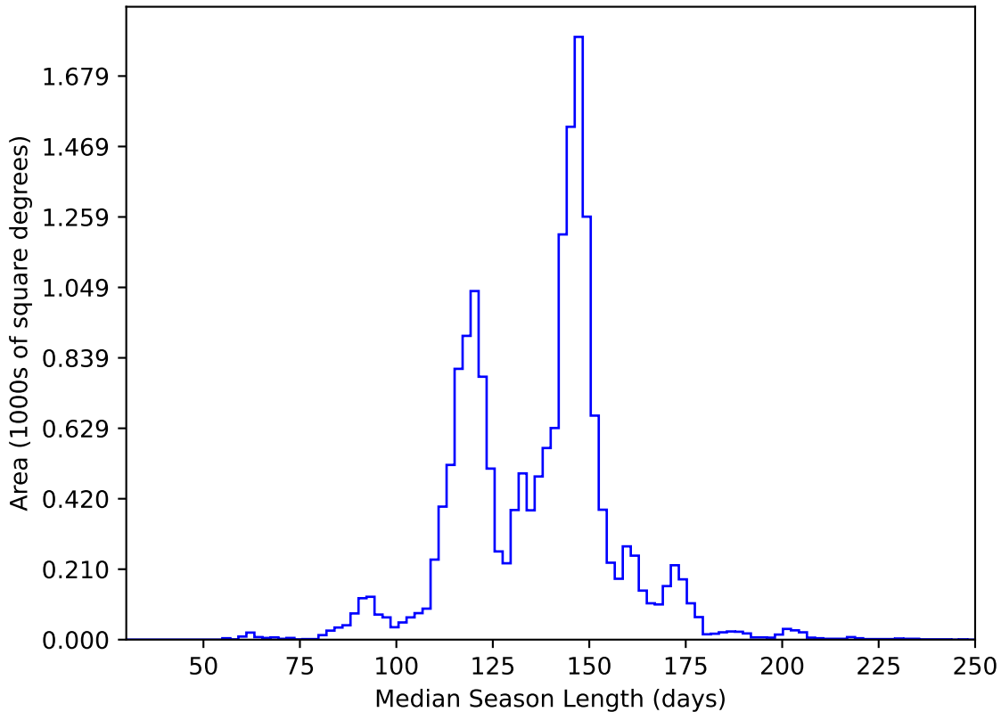
ddf_acor_sf25_lsf30_lsr10_v3.4_10yrs WFD y band: Median Season Length
