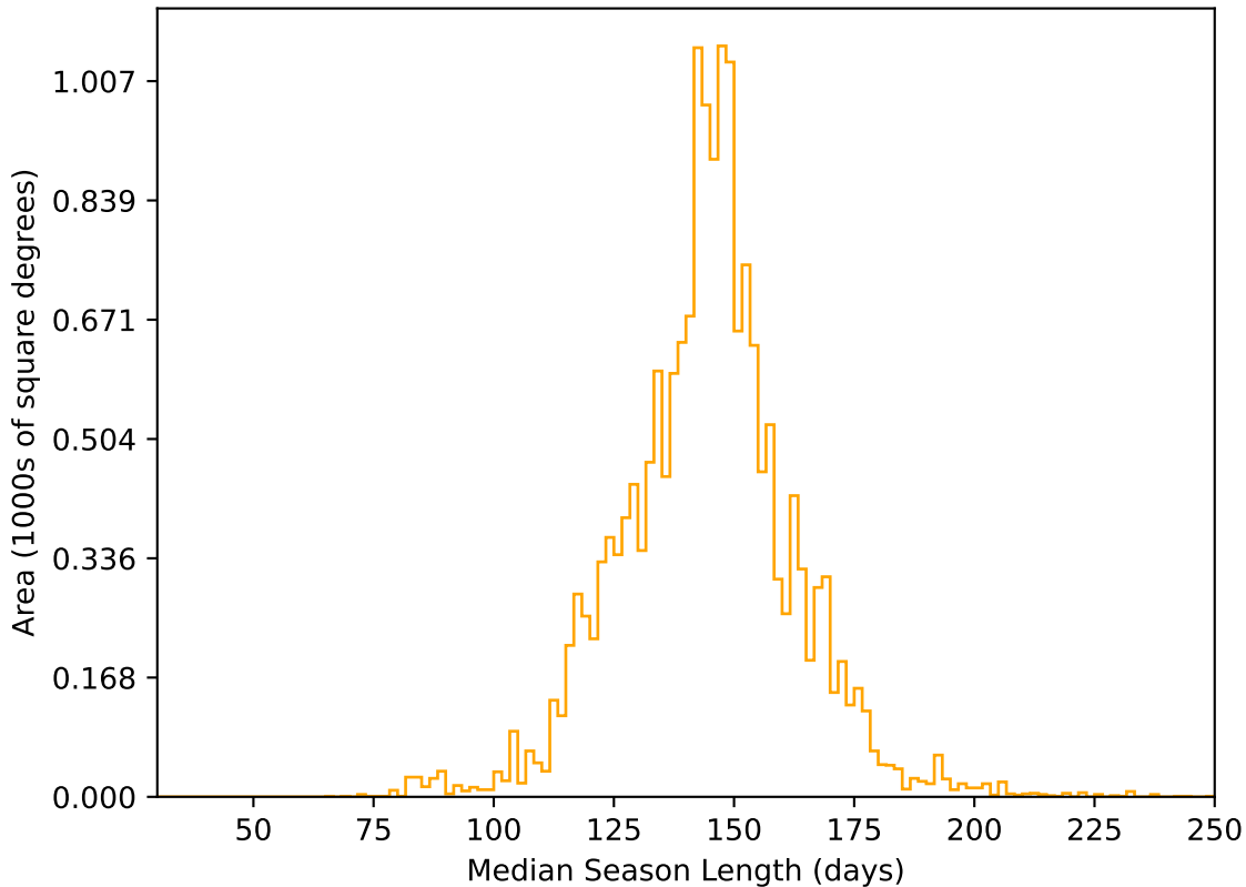
ddf_acor_sf25_lsf30_lsr10_v3.4_10yrs WFD r band: Median Season Length
