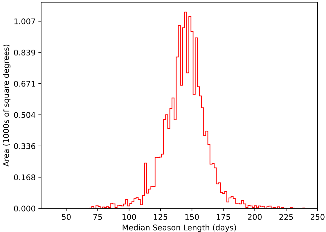
ddf_acor_sf25_lsf30_lsr10_v3.4_10yrs WFD i band: Median Season Length
