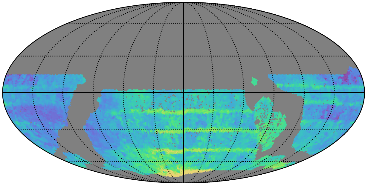
ddf_acor_sf25_lsf30_lsr10_v3.4_10yrs WFD all bands: Median Season Length
